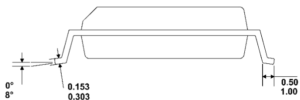
LEFT-SIDE VIEW
